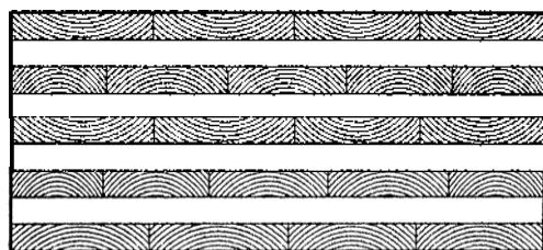
Figure A1.4: Principal structure of a solid wood slab with 9 layers.
