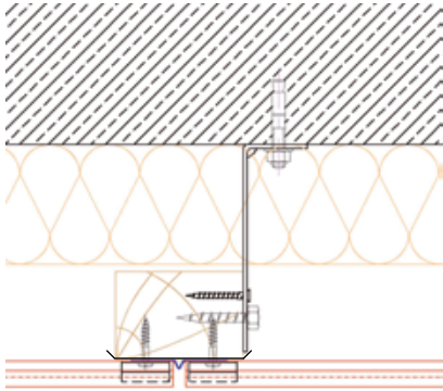
JOINT VERTICAL
