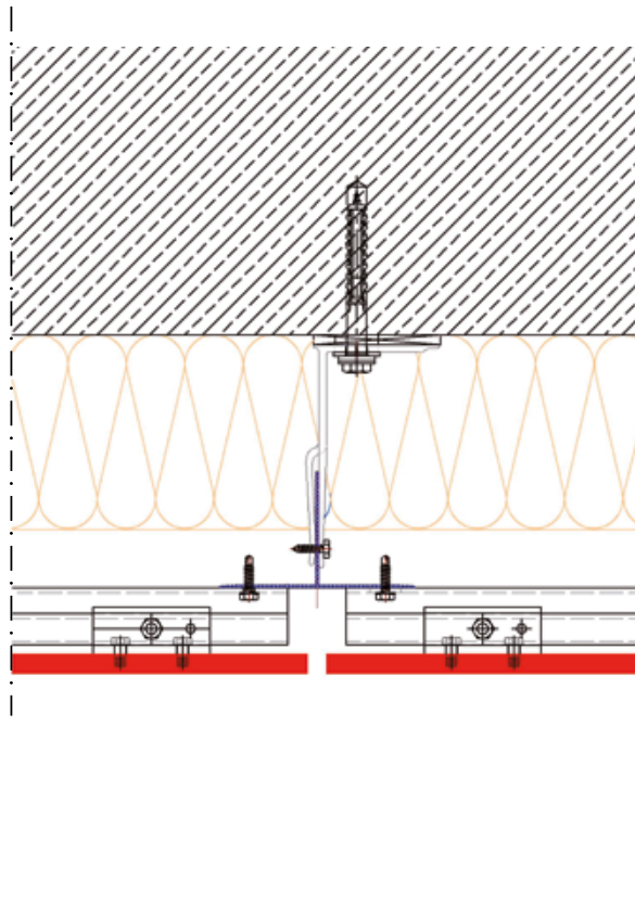
JOINT VERTICAL
