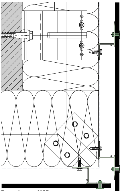
External corner A105
