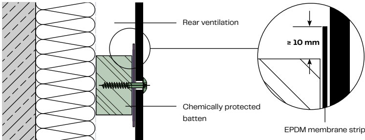
Central supporting batten A108
